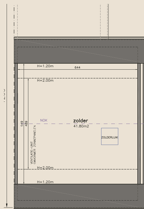
Zolder
