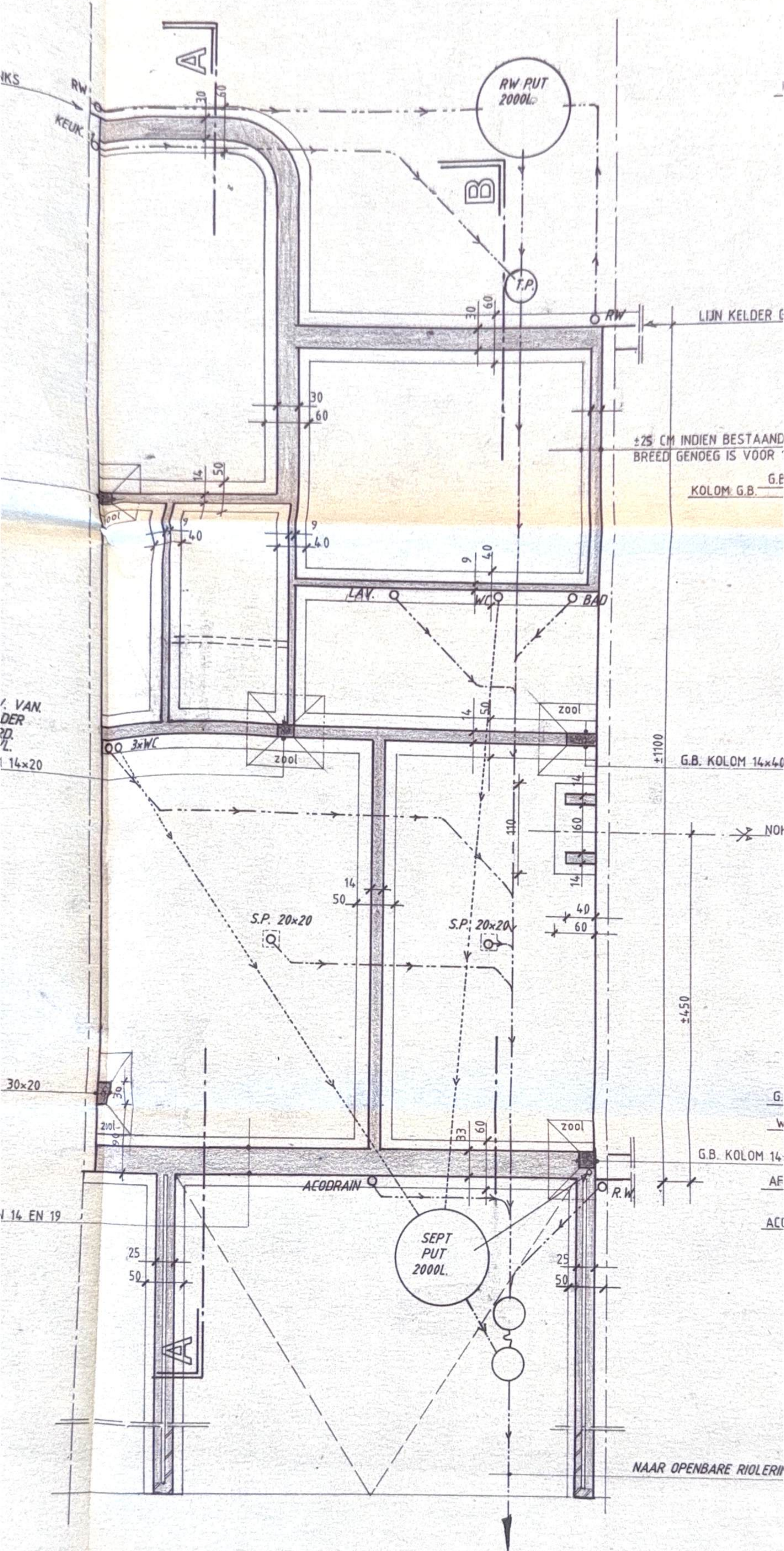
funderings- & rioleringsplan
